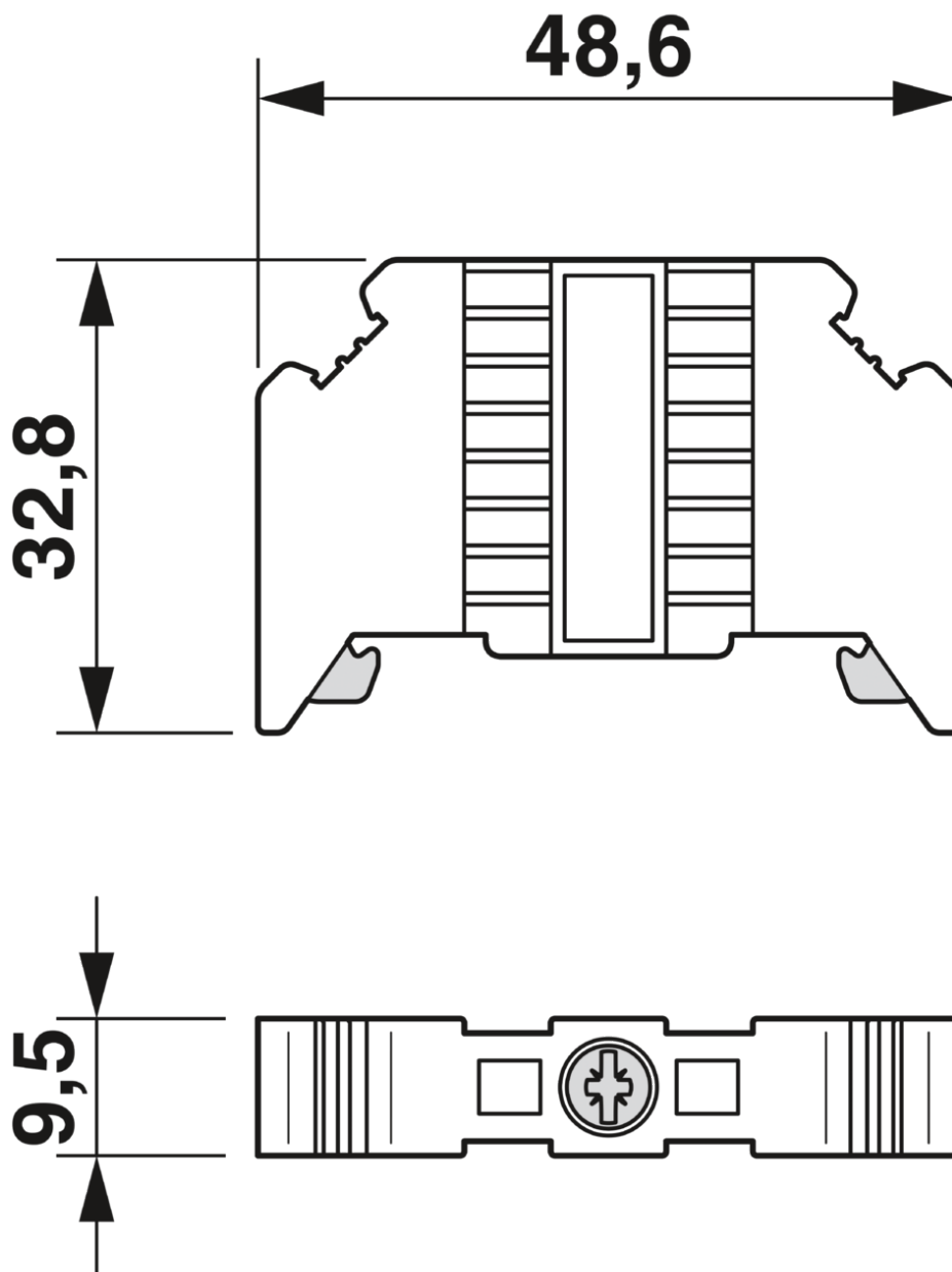
Dimensional drawing
